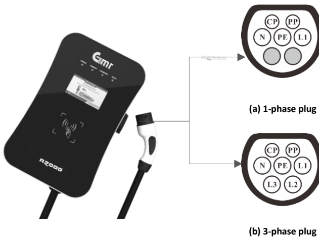
Fig. 3-5 Schematic diagram of Type 2 plug on M3W series products
