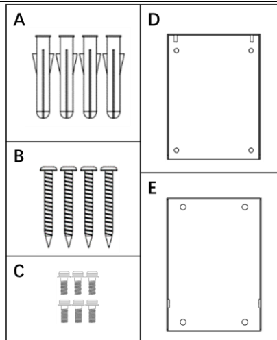
Fig. 5-1 Wall-mounting accessories
