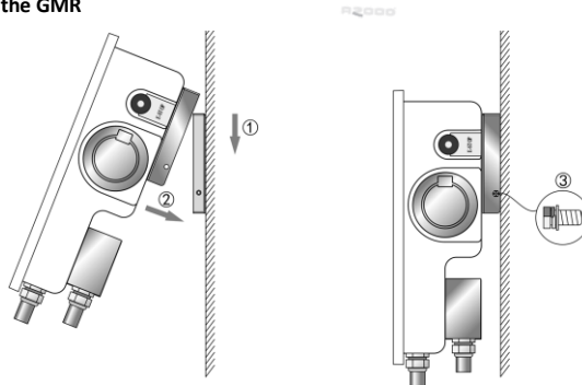
Fig. 5-7 Fix the GMR on the wall
