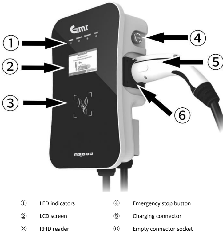
Fig. 6-1 HMI of GMR
