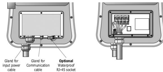
Fig. 5-6 Wiring the input power cable
