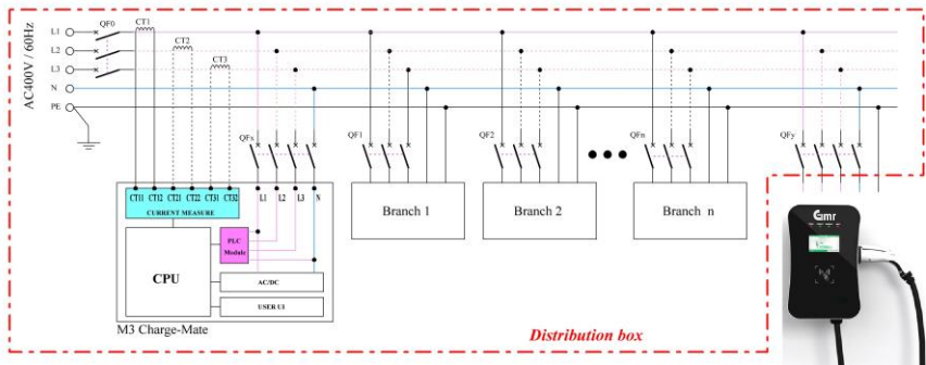
Fig. 8-5 System wiring diagram
