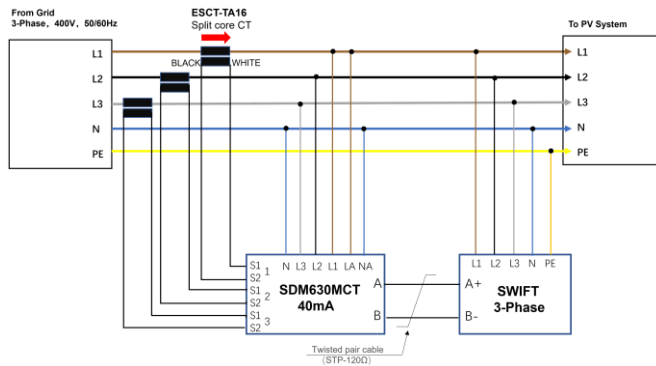
Fig. 8-3 Wiring diagram for 3 Phase system
