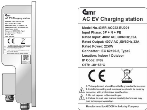
Fig. 4-4 The location and content of the nameplate
