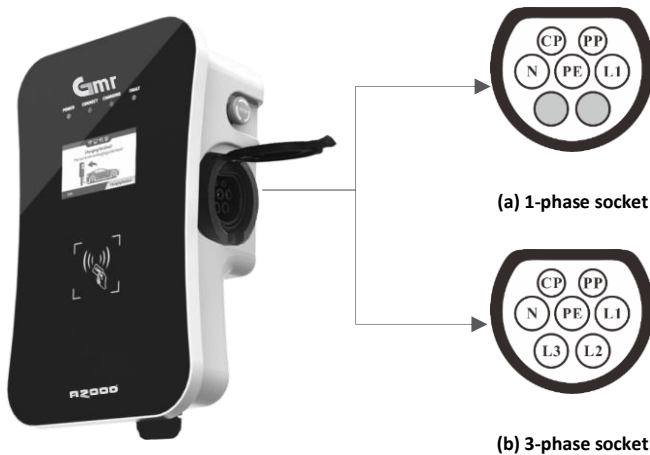
Fig. 3-3 Schematic diagram of Type 2 socket on GMR M3B series
