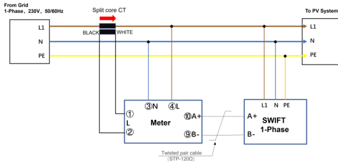
Fig. 8-2 Wiring diagram for 1 Phase system
