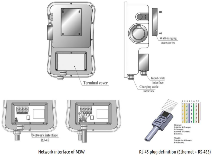
Fig. 8-1 Terminal of GMR
