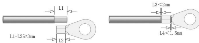
Fig. 5-5 Peeling cables and press terminals
