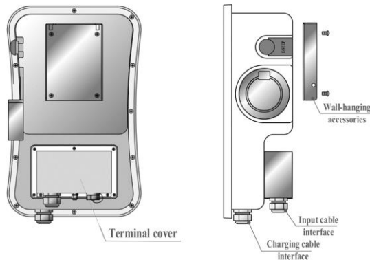
Fig. 5-4 Fix the wall-hanging accessories
